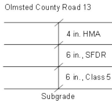
Figure 5: Olmsted County Road 13 Section
