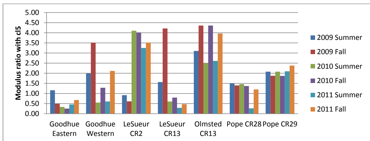
Figure 38: Modulus Ratios
