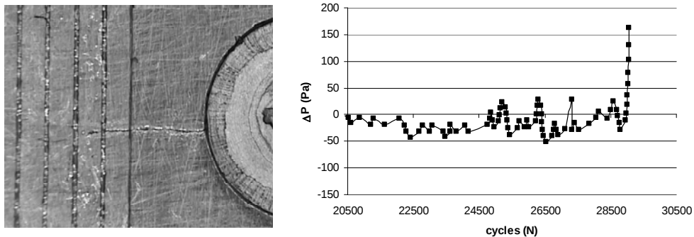
Figure 2: Fatigue Crack Crossing Into CVM Galleries; (Pressure increase caused by crack reaching a gallery is clearly indicated)
