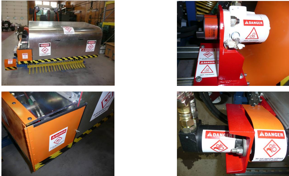
Figure 39: Safety labels
