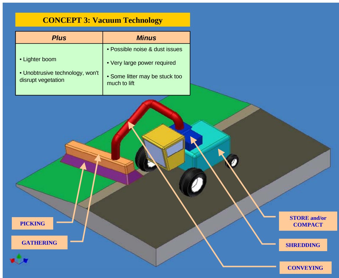
Figure 6: Vacuum technology
