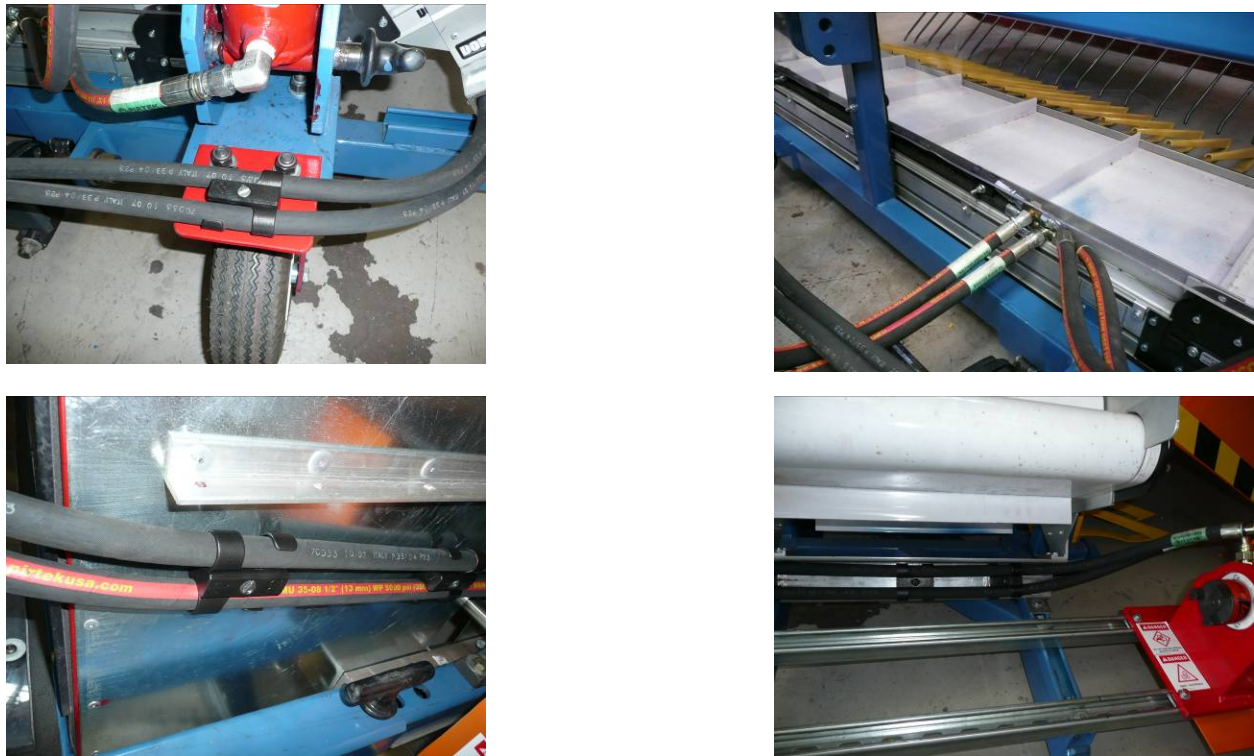
Figure 41: Hoses routing
