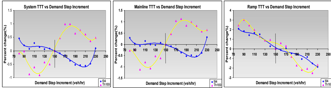
Figure 5.3 Effect of parameter Ramp demand Increment on Performance MOEs
