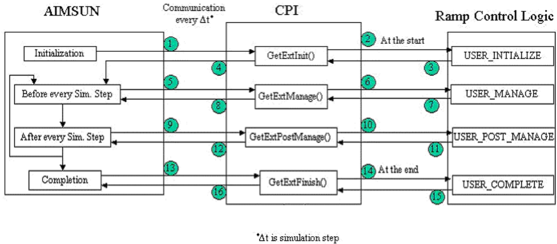
Figure 3.5 CPI interactions with the Simulator and the Ramp Control Logic
