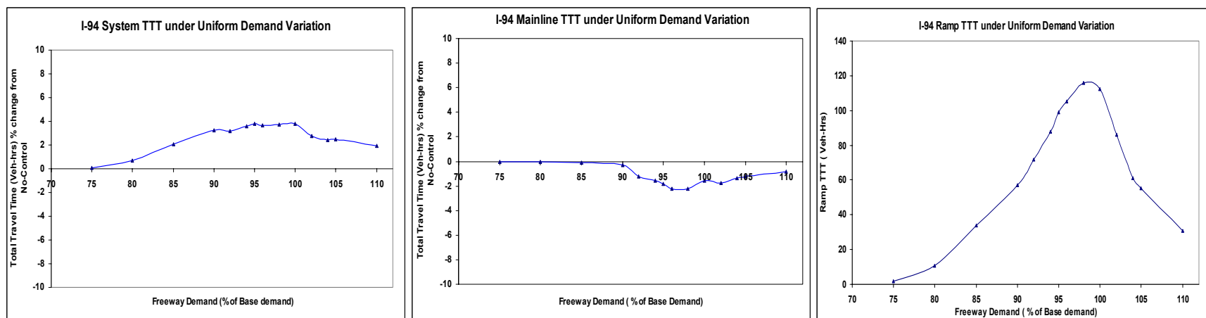
Figure 6.2 Effect of Uniform Demand Variation on I-94
