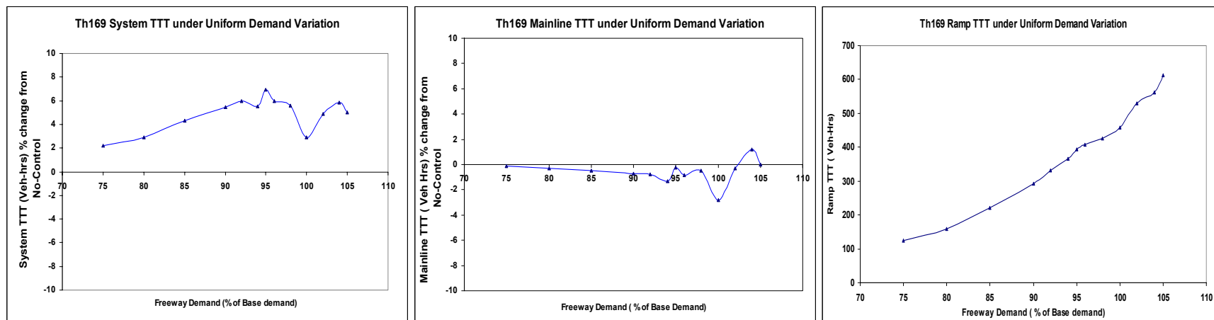
Figure 6.1 Effect of Uniform Demand Variation on TH-169
