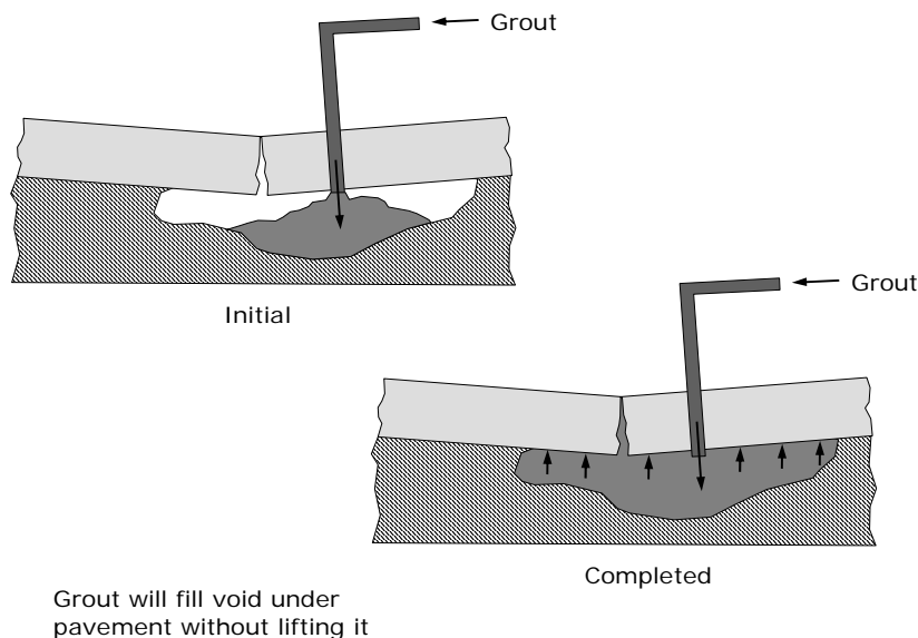
Figure 11.1 Injecting grout.
